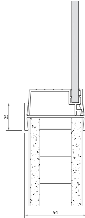
Transom Detail Solid - Single Offset Glazed
