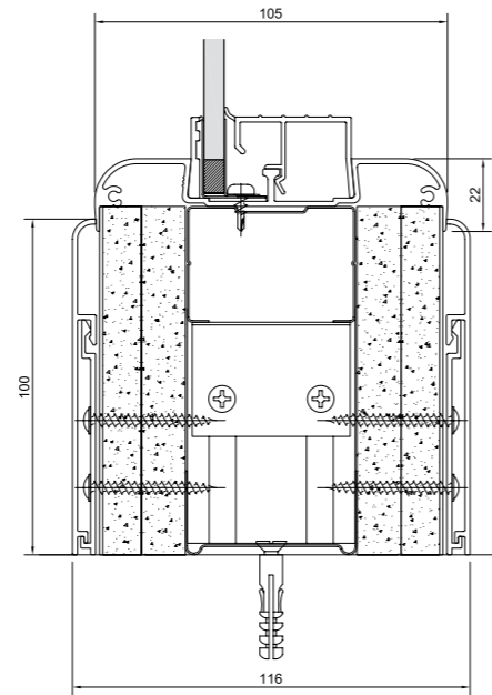
Mullion - Door/Double Glazed (30 mins Fire Rated)
